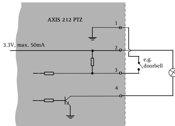
Terminal Connectors - Schematics
