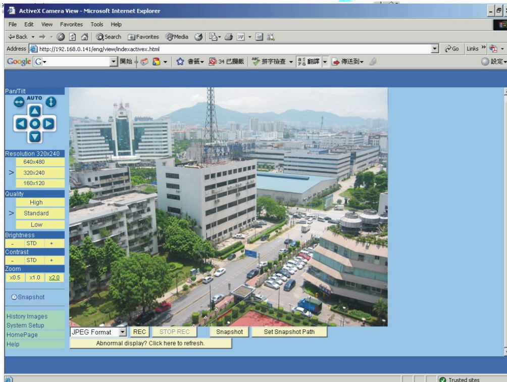
Figure 22 Video webpage
