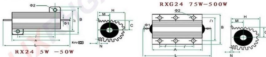
physical dimension
